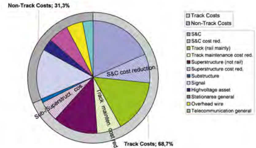
Figure 9-1: Example of maintenance cost distribution from Banverket. For simplicity a possible 30% cost reduction has been demonstrated by assuming an equal 30% reduction in annual maintenance cost of the largest cost groups.
