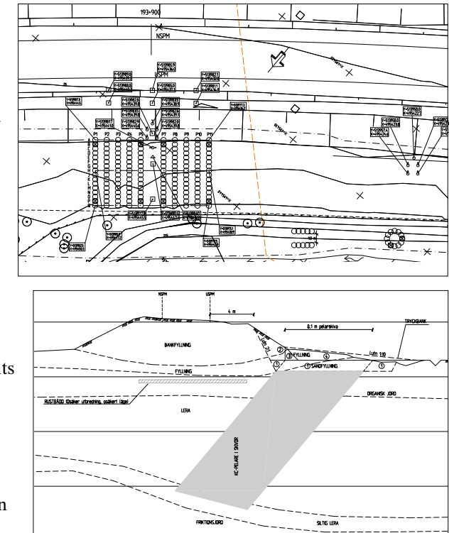
Figure 4.2.1-4: Top: Plan of the installation of columns and column walls (panels) at the Torp
