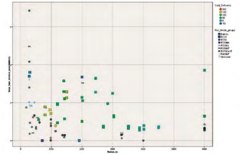
Figure 5.1.1-1: 45^\circ Wear rate for different rail grades as a function of curve radius.
