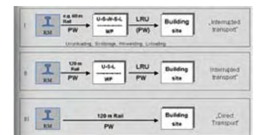
Figure 5.7-1: Transportation modes (RM: Rolling Mill, PW: Public Wagon, WP: Welding plant, LRU: Long Rail Unit)
