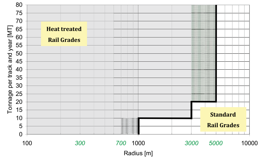
Figure 5.2-2: Revised rail grade selection recommendation based on rail radii and operational volume
