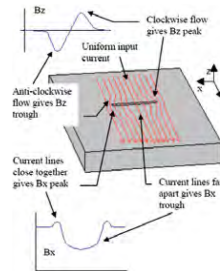
Figure 5.5.1-1: ACFM concept
