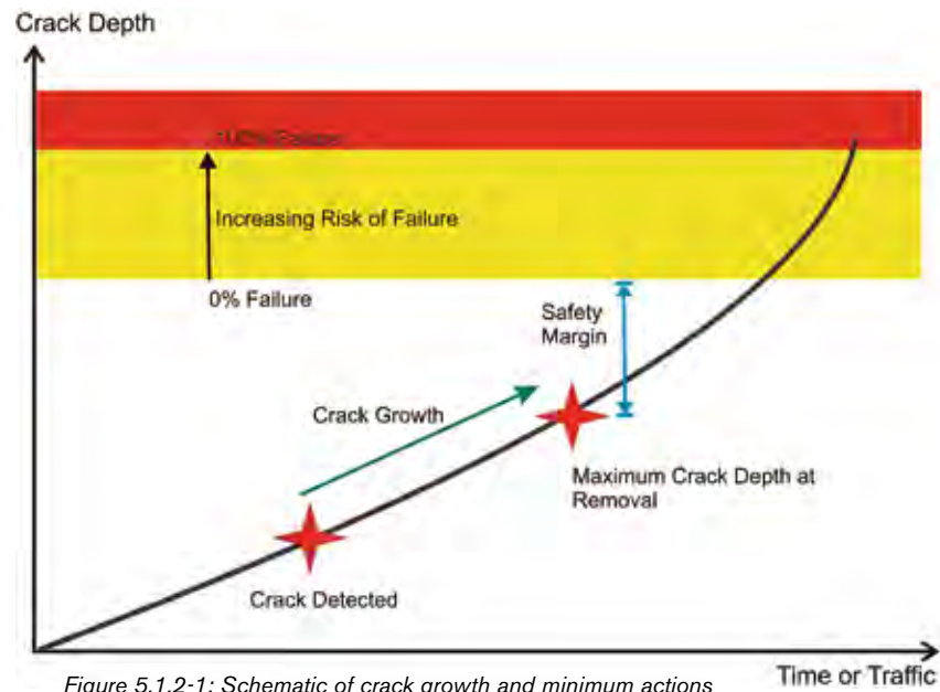
Figure 5.1.2-1: Schematic of crack growth and minimum actions
