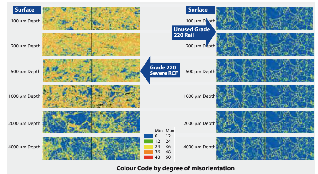
Figure 5.4.4-3: Comparison of grade 220 rails in untrafficked and trafficked conditions using EBSD
