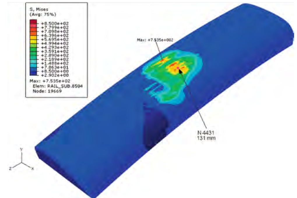
Figure 5.4.3-2: FE-simulation of the DB test rig. Von Mises stress evaluated during the fifth load passage.
