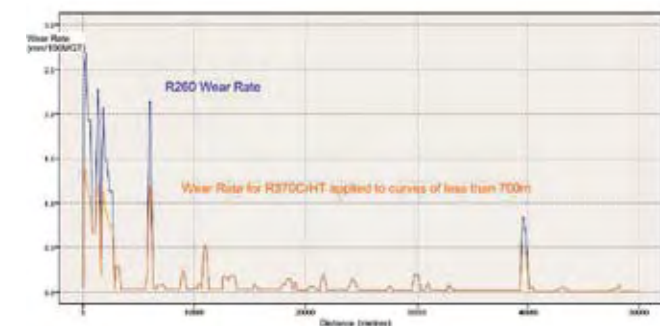
Figure 5.1.1-3: Predicted effect of premium grade rail steels on 45^\circ wear for a 120 km route
