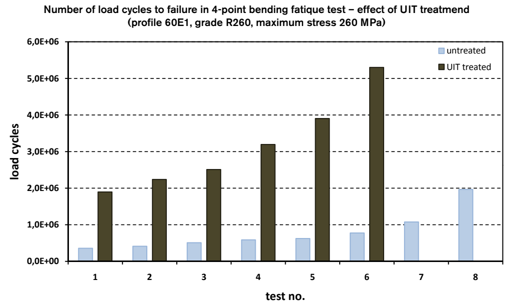
Figure 5.6.1-2: Results of fatigue tests of aluminothermic welds (rail grade R260).
